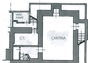
Piano interrato Basement
